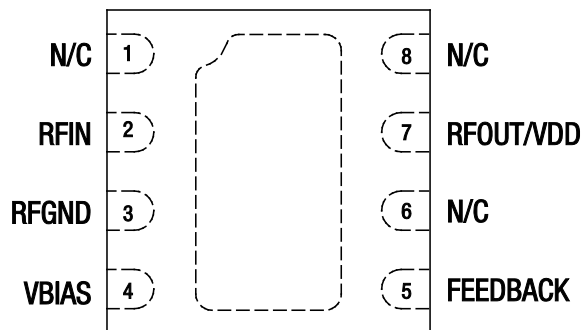
Figure 2. SKY67110-396LF Pinout – 8-Pin DFN (Top View)
