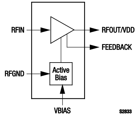
Figure 1. SKY67110-396LF Block Diagram
