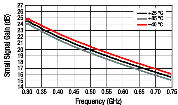
Figure 4. Narrowband Gain Response vs Frequency Over Temperature
