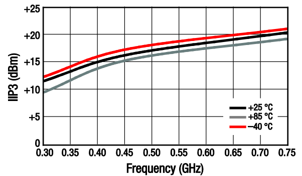
Figure 12. IIP3 vs Frequency Over Temperature
