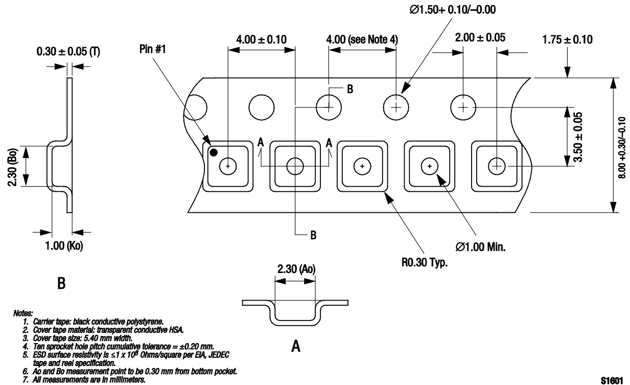
Figure 25. SKY67110-396LF Tape and Reel Dimensions
