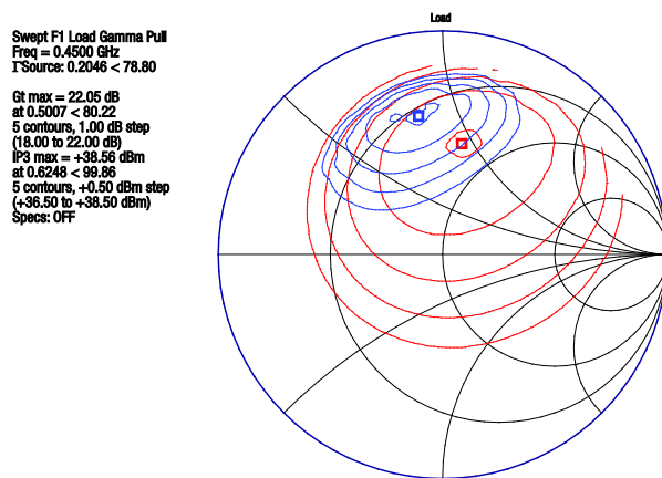
Figure 18. OIP3 Load Pull @ 0.45 GHz, 5 V, 76 mA (Input Load = NF Min., -20 dBm/Tone, 5 MHz Spacing)
