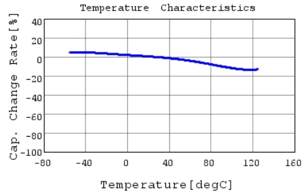
GRT155R70J223KE01 C-Temp. capchange, DCOV, 1
