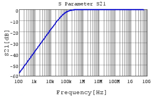
GRT155R70J223KE01 S21 DCOV, 25degC
