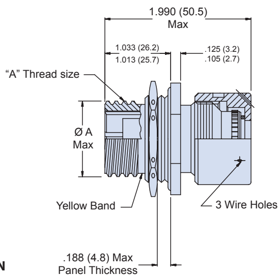
04 - JAM NUT MOUNT RECEPTACLE WITHOUT BACKSHELL M28876/11 • 180-040 (-04)
