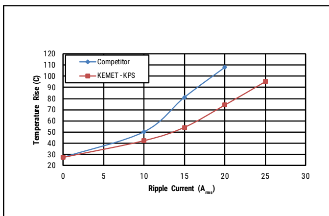
Ripple Current ( A_{rms} ) 2220, 22 \mu F, 50 V
