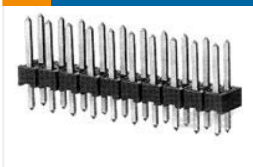
TE Part #5-146257-4 08 MODII HDR DRST B/A .100CL L
