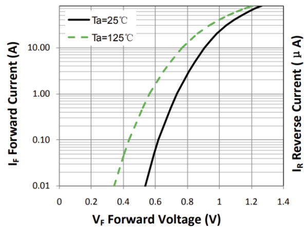
Figure 1. Forward Characteristic(typ.)
