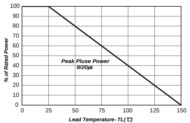
Fig2.Power Derating
