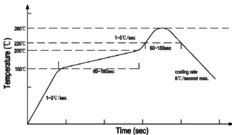
Reflow -curve
