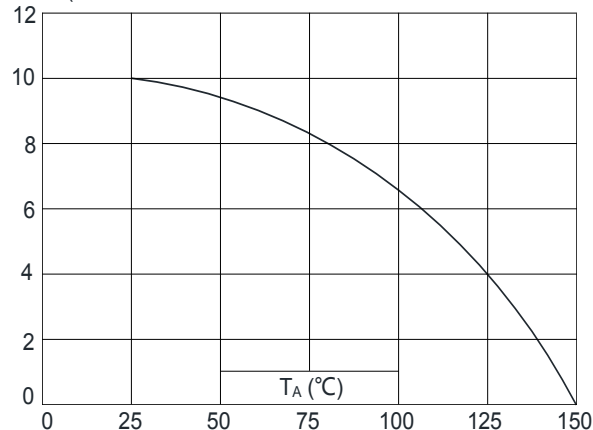
-I_D(A)
