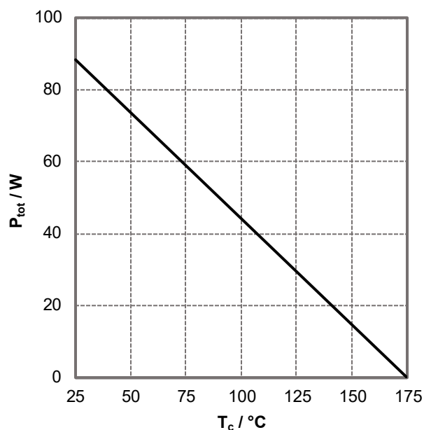
Figure 3. Power Derating
