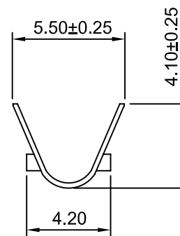
SEC:C-C
