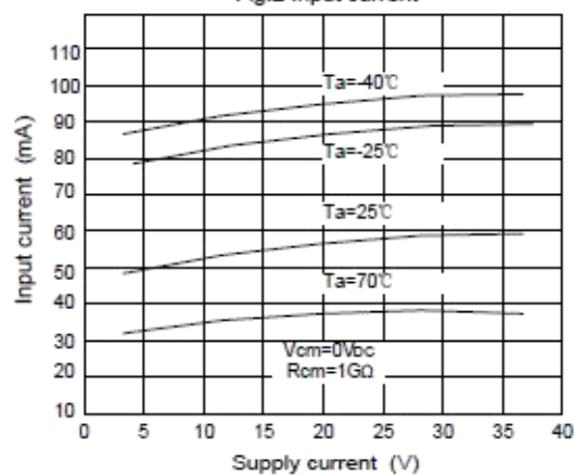
Fig.2 Input current
