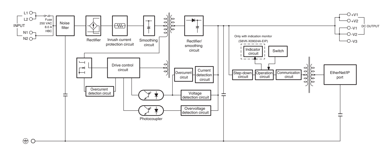
S8VK-X12024-EIP
