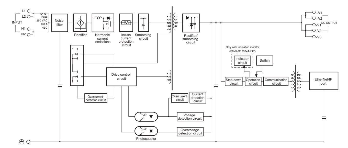
S8VK-X12024-EIP
