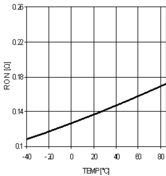
Fig.8 Hi,Low-Side On-resistance
