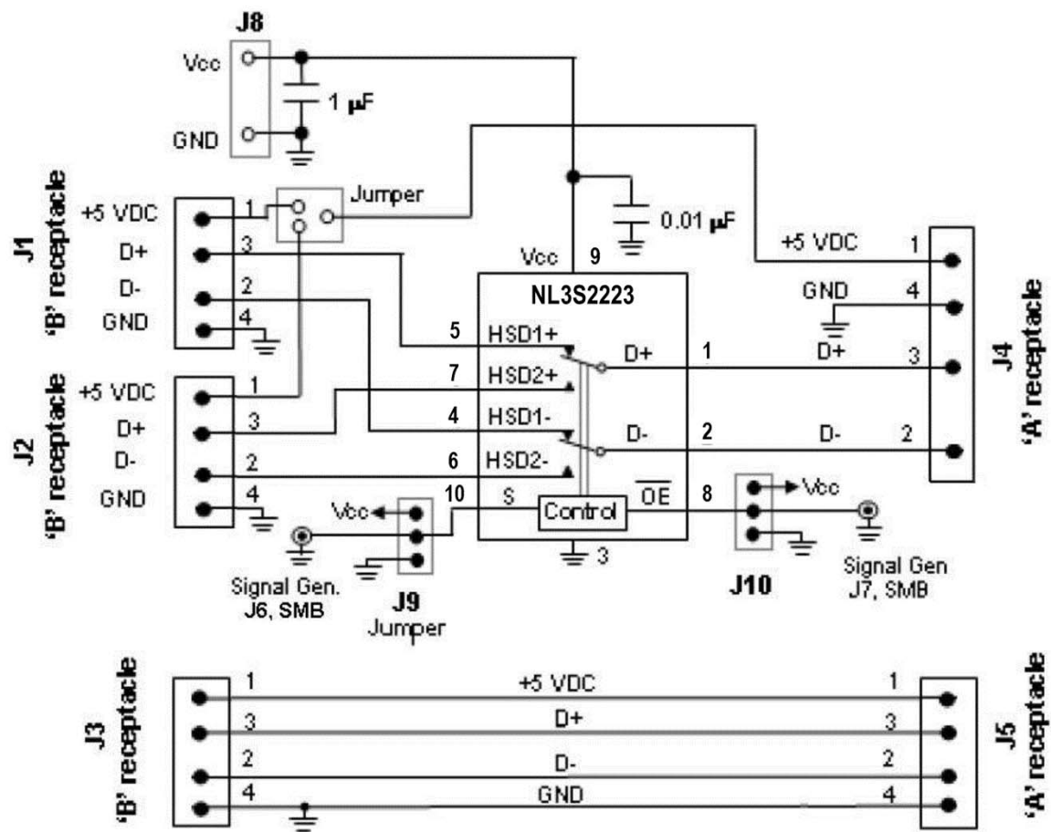
Figure 7. Board Schematic
