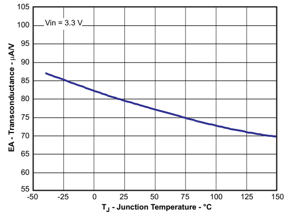
Figure 8. Transconductance (Soft-Start) vs Junction Temperature
