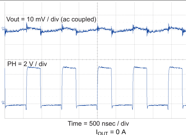
Figure 45. Output Ripple
