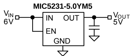
5V Linear Regulator Application
