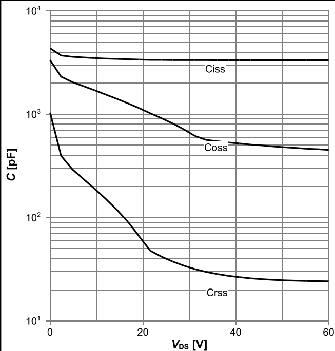
Diagram 11: Typ. capacitances
