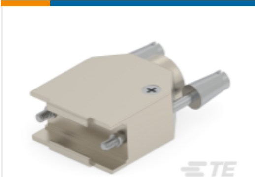
TE Part #5-2198617-1 Pltd Plastic Backshell 9 way Str, KIT
