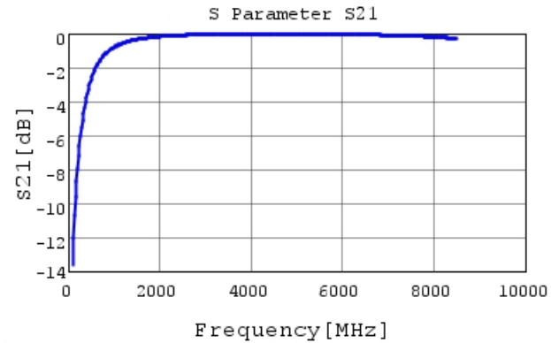
GCQ1555C1H3R4WB01 S21 DCOV, 25degC
