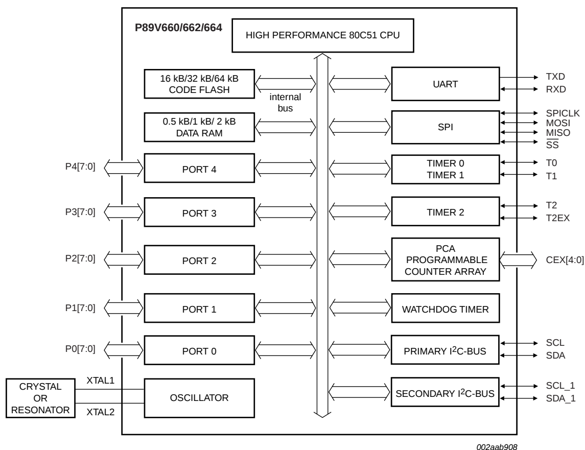
Fig 1. Block diagram
