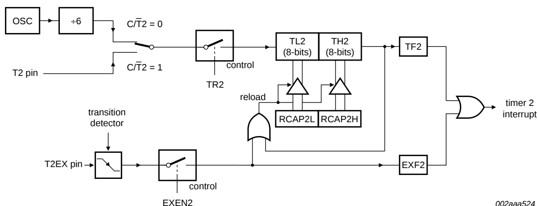
Fig 19. Timer 2 in Auto-reload mode (DCEN = 0)
