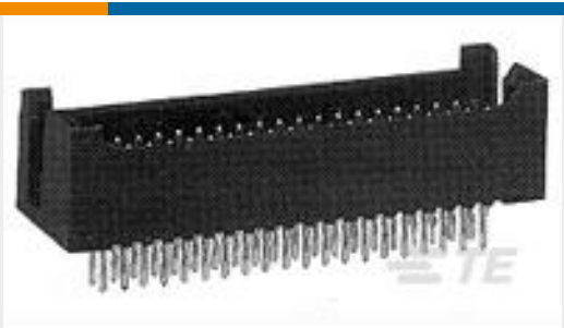
TE Part # 5-534978-8 50 MODII 2PC HDR DR W/HLDWN, ROHS
