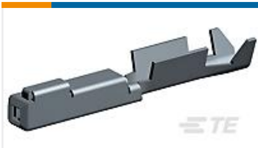
TE Part #2040168-1 0.64 RCPT SEALED TIN STRIP(L SIZE)
