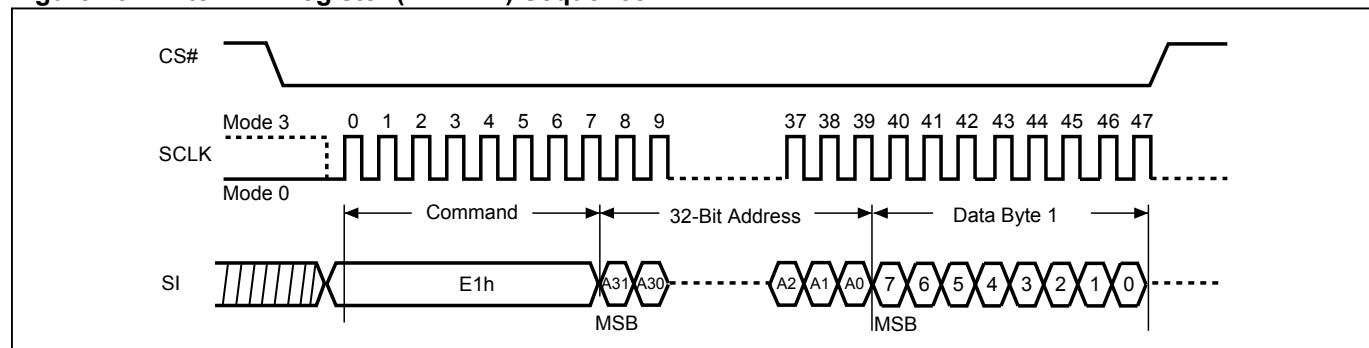
Figure 75. Write DPB Register (WRDPB) Sequence
