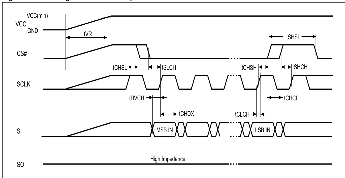
Figure 89. AC Timing at Device Power-Up
