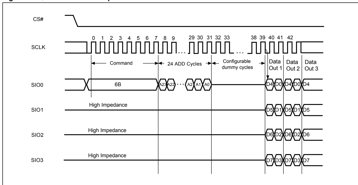
Figure 33. Quad Read Mode Sequence
