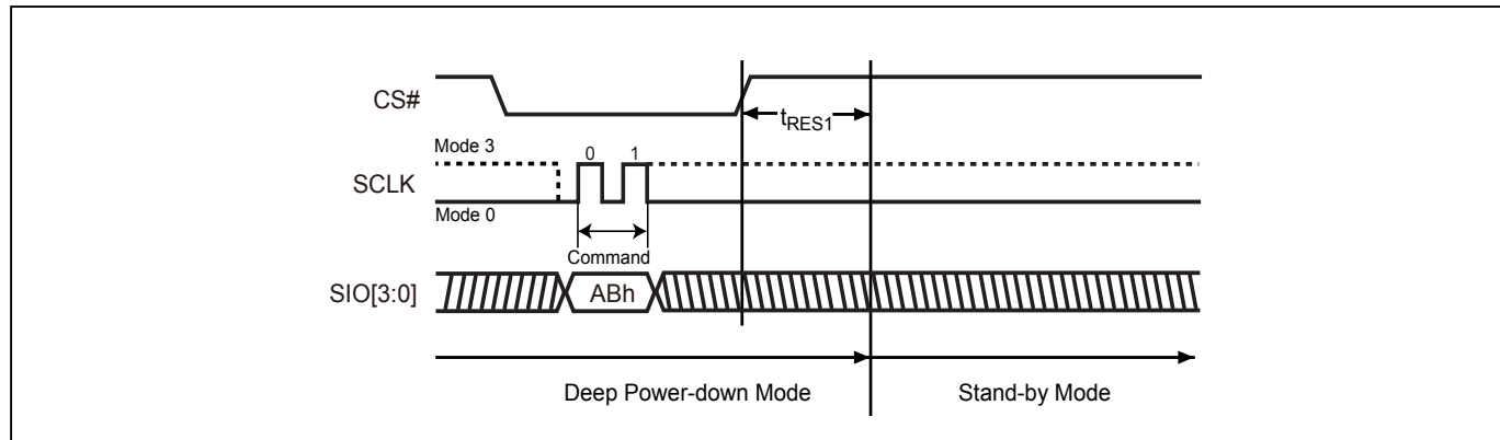
Figure 17. Release from Deep Power-down (RDP) Sequence (QPI Mode)
