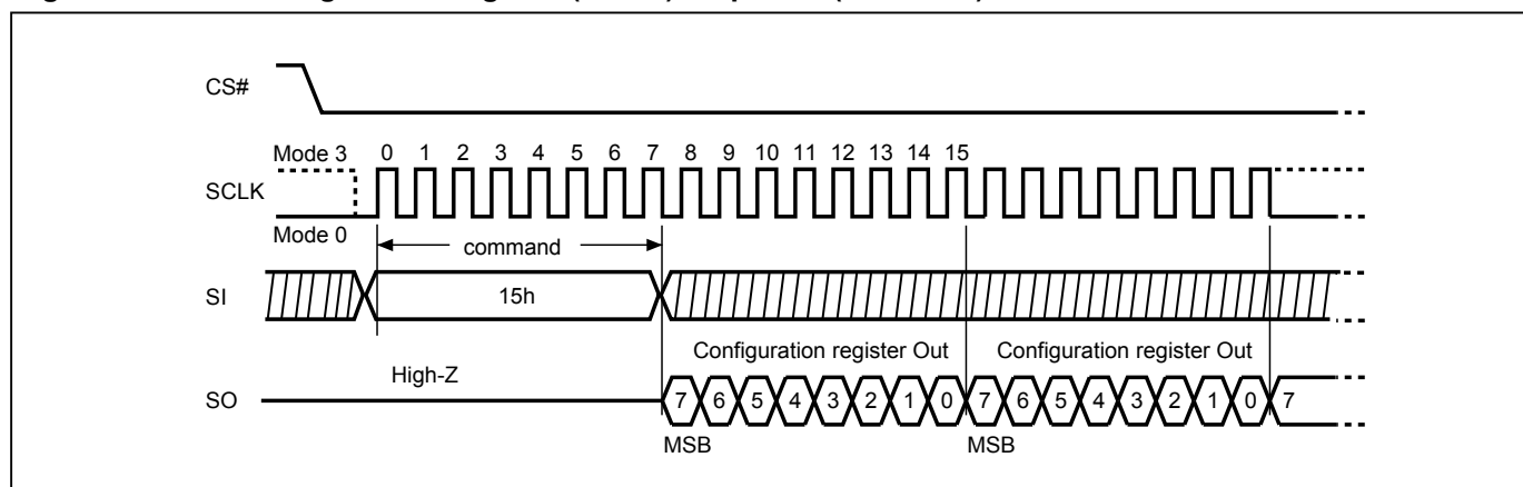
Figure 21. Read Configuration Register (RDCR) Sequence (SPI Mode)
