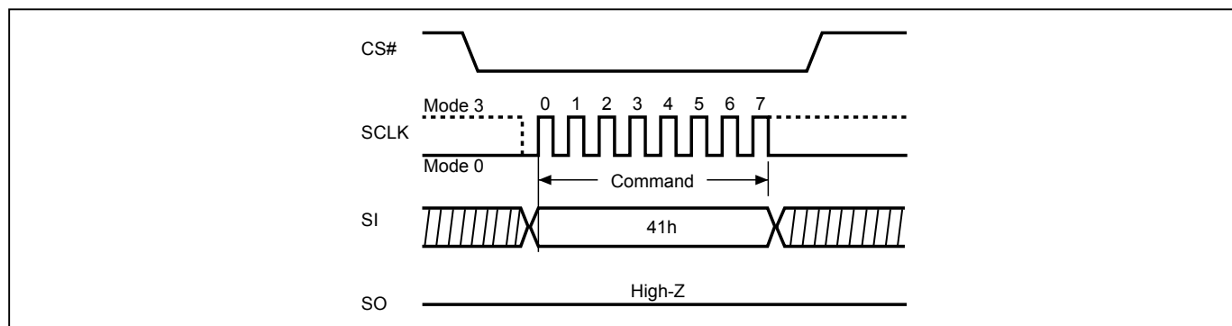
Figure 11. Factory Mode Enable (FMEN) Sequence (SPI Mode)
