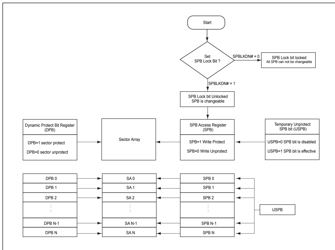
Figure 68. Advanced Sector Protection Overview
