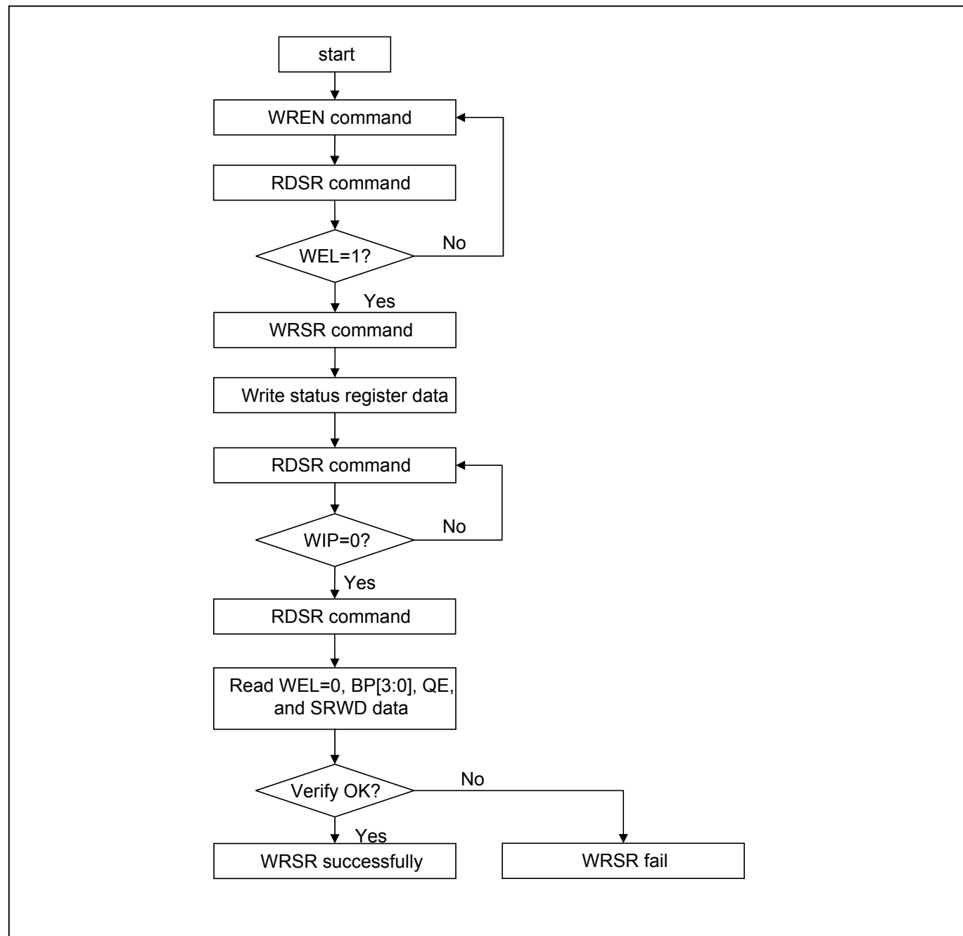
Figure 27. WRSR flow
