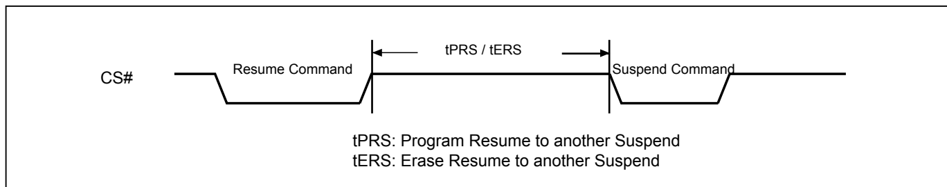
Figure 78. Resume to Suspend Latency
