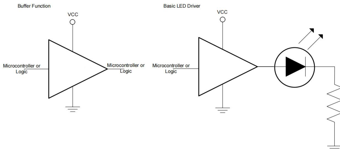
Figure 5.1: Application Schematic
