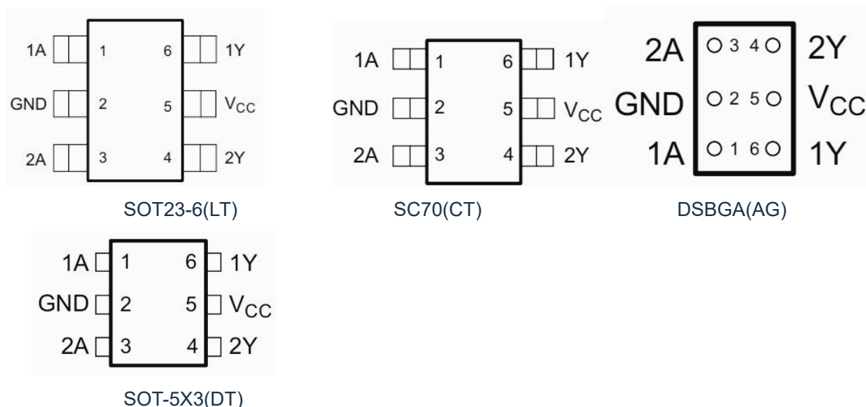
Figure 2.1 Top View
