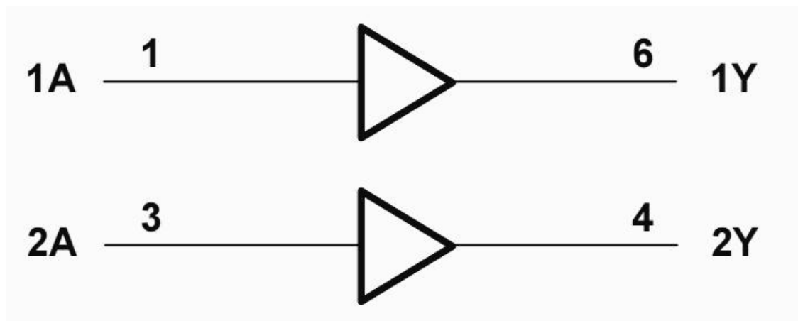
Figure 3.1: 74LVC2G34 Logic Diagram
