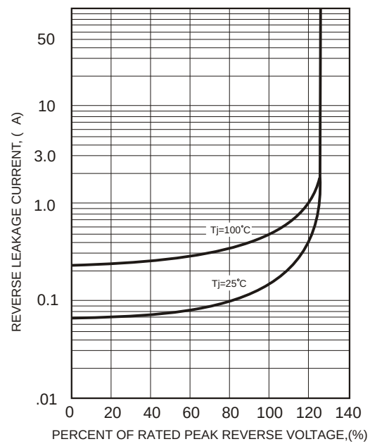
FIG.3-Typical Reverse Characteristics
