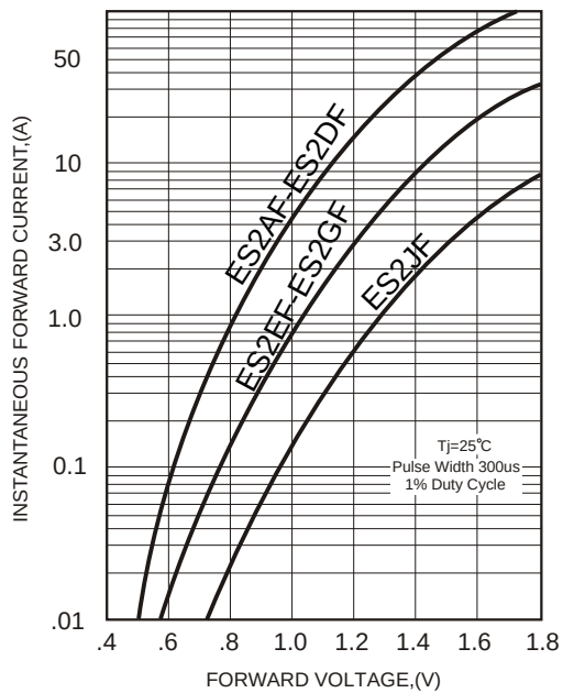
FIG.2-Typical Forward Characteristics
