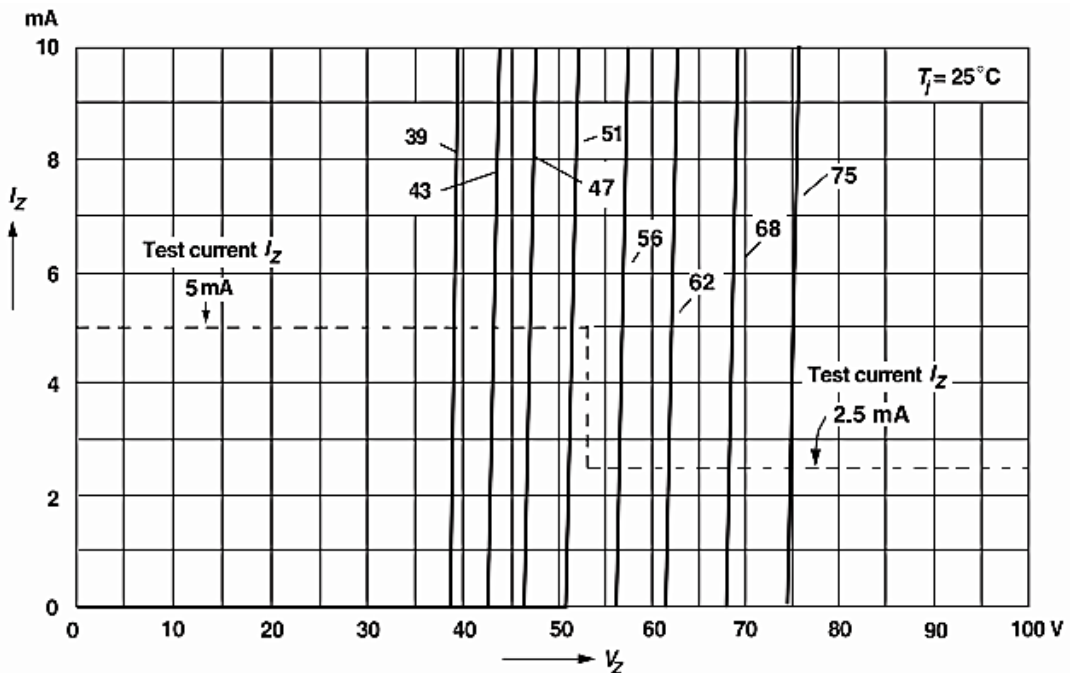
Figure 16. Breakdown Characteristics
