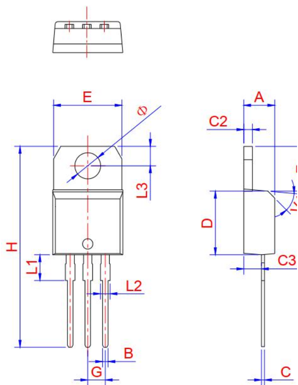
TO-220B Non-Ins
