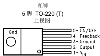
LM2576T-XX 或 LM2576HVT-XX
