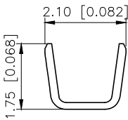
SECTION:B-B SCALE:1:1
