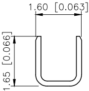
SECTION:C-C SCALE:1:1
