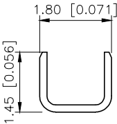
SECTION:A-A SCALE:1:1
