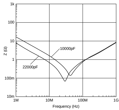
GR7 Series
