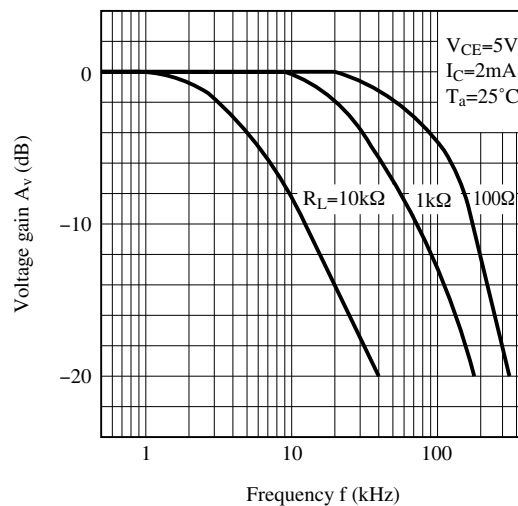
Fig.14 Frequency Response
