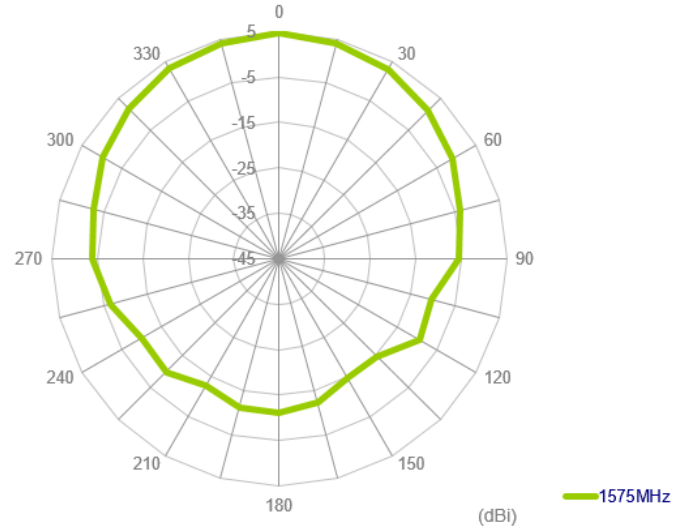
YZ Plane ( \phi=90^\circ , \Theta=0\sim360^\circ )
