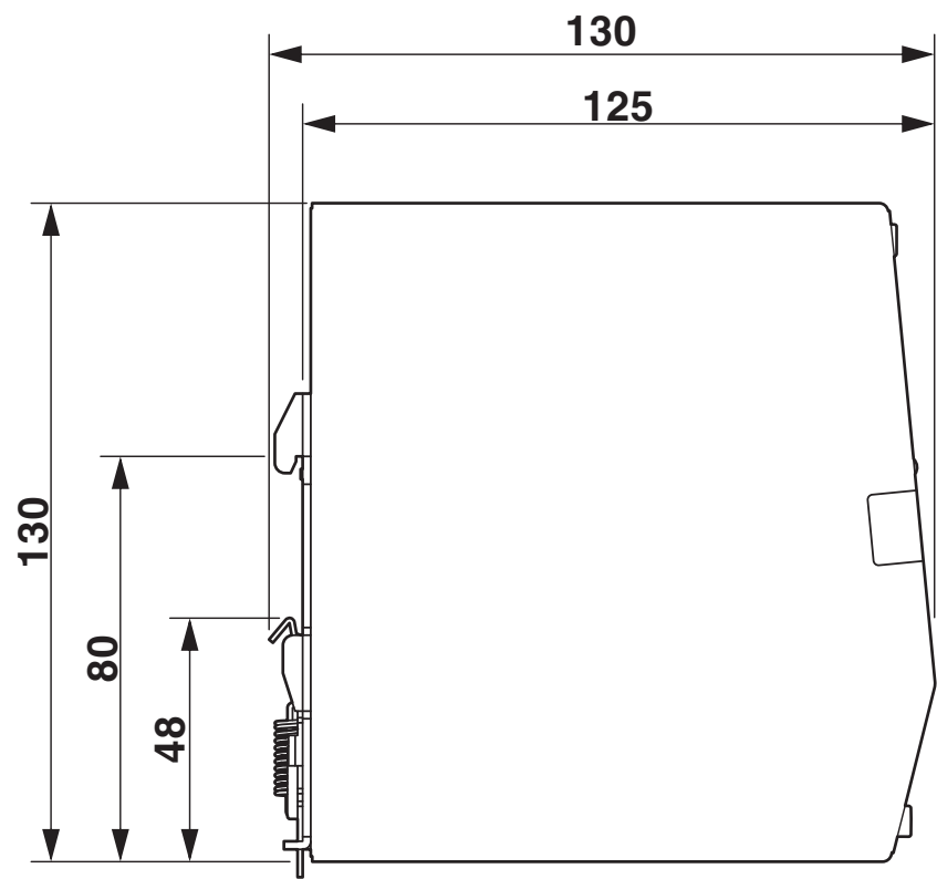
Dimensional drawing
