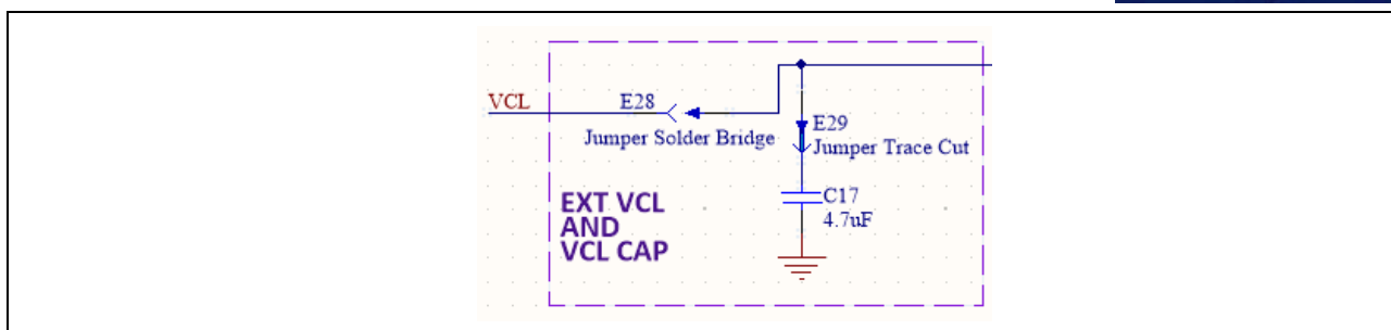
Figure 28. External Capacitor to VCL Circuit
