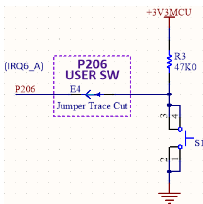
Figure 15. User Switch Circuit
