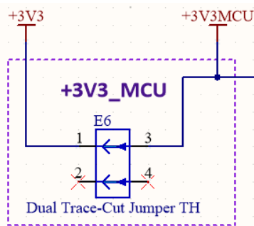
Figure 11. MCU Current Measurement Circuit
