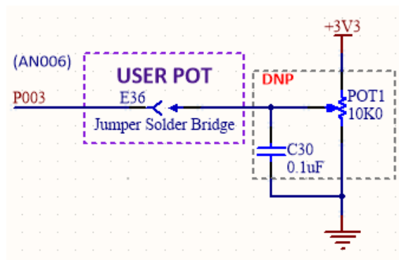
Figure 25. User Potentiometer Circuit
