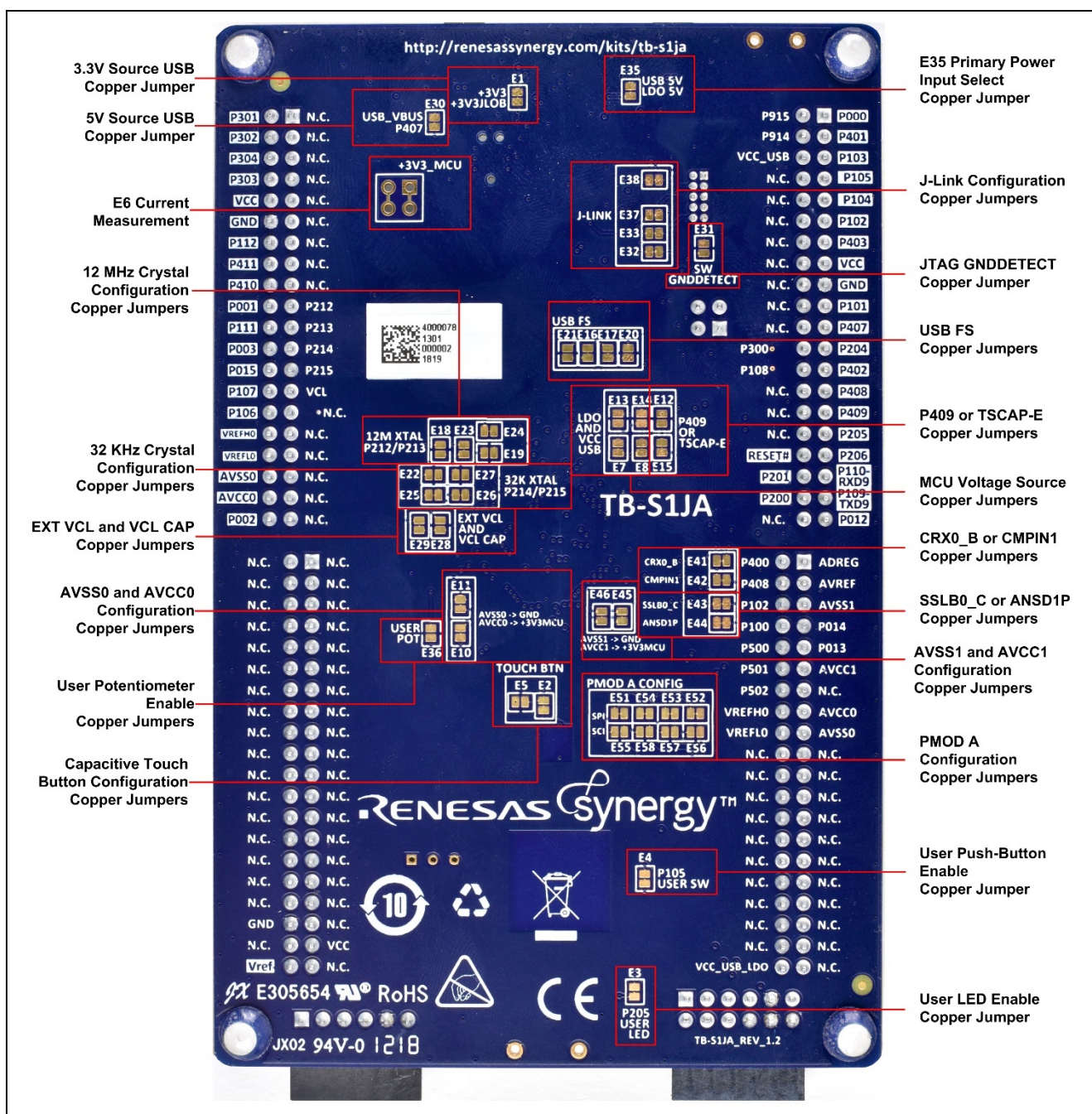
Figure 2. TB-S1JA Bottom Side
