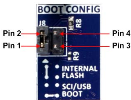
Figure 27. Boot Config Jumper J8
