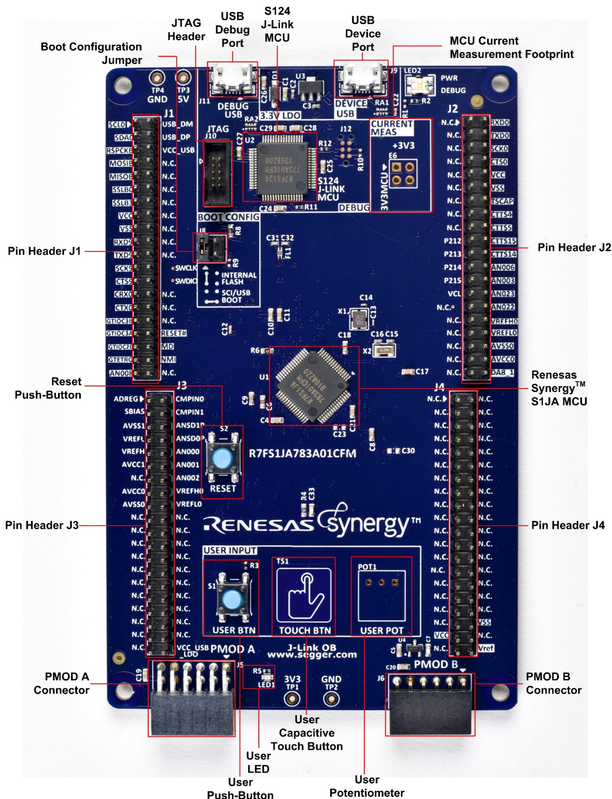
Figure 1. TB-S1JA Top Side
