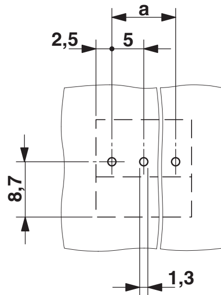
Dimensional drawing
