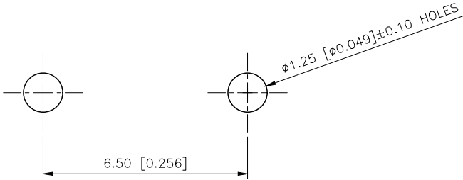
P.C.B MOUNTING HOLES
