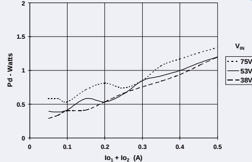
Power Dissipation vs. Total Output Current ( I_{O1} + |I_{O2}| )
