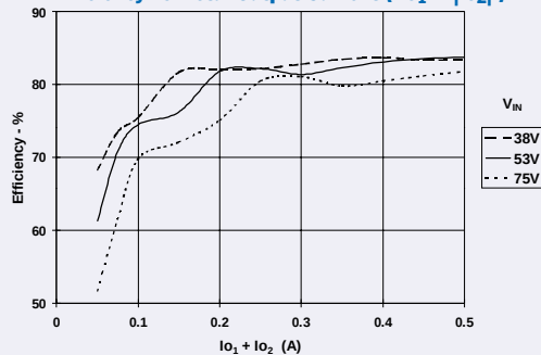
Efficiency vs. Total Output Current ( I_{O1} + |I_{O2}| )
