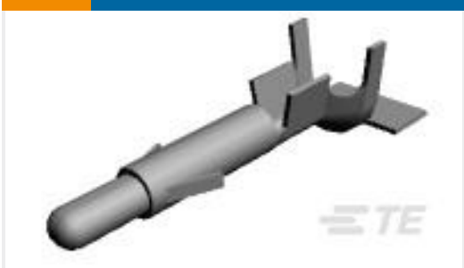
TE Part #350707-7 UMNPL SPLIT PIN 20-14 AUBR L/P
