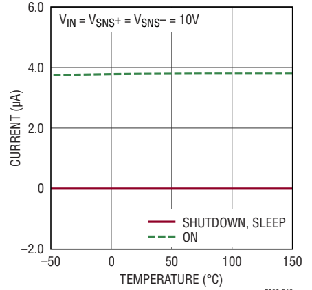
SNS^- Supply Current vs Temperature
