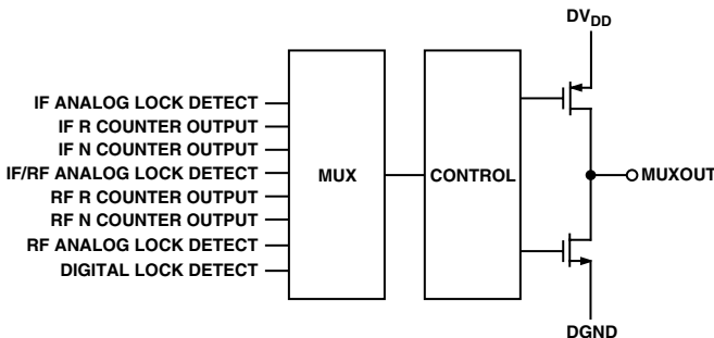
Figure 6. MUXOUT Circuit
