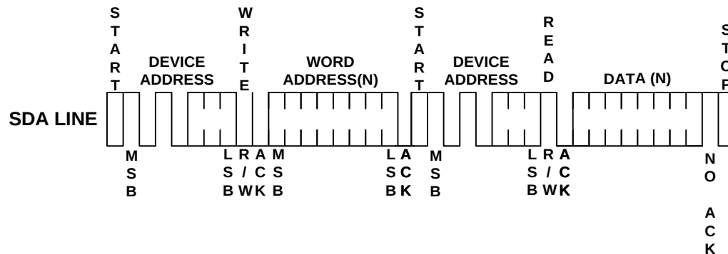
Figure 9: Random Read
