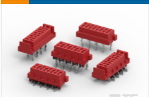
TE Part #7-215079-8 Female-on-Board Connector, Top Entry
