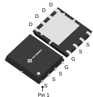
DFN5X6-8L (DFN-5(5x6))
