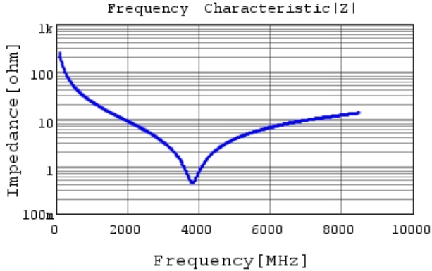
GRM0335C2A6R5BA01 |Z| DCOV, 25degC
