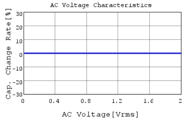
GRM0335C2A6R5BA01 C-AC Voltage capchange, Dc
