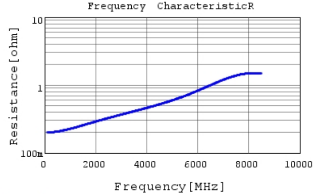
GRM0335C2A6R5BA01 R DCOV, 25degC
