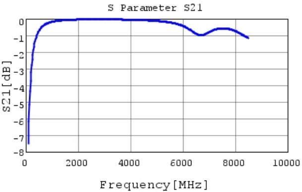
GRM1555C2A7R4CA01 S21 DC0V, 25degC
