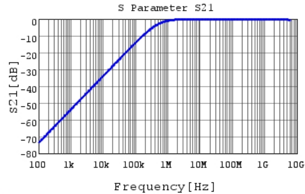
GCJ188L81H332KA01 S21 DC0V, 25degC
