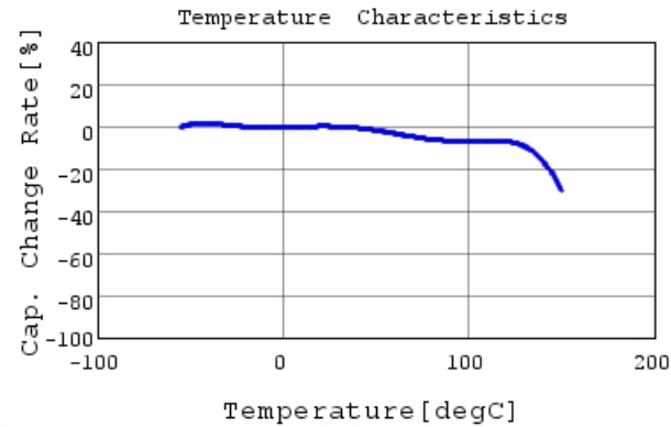
GCJ188L81H332KA01 C-Temp. capchange, DC0.0V,
