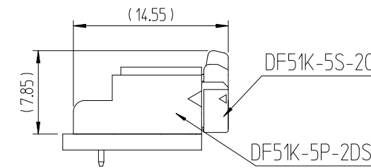
ENGAGEMENT FIGURE (2:1)
