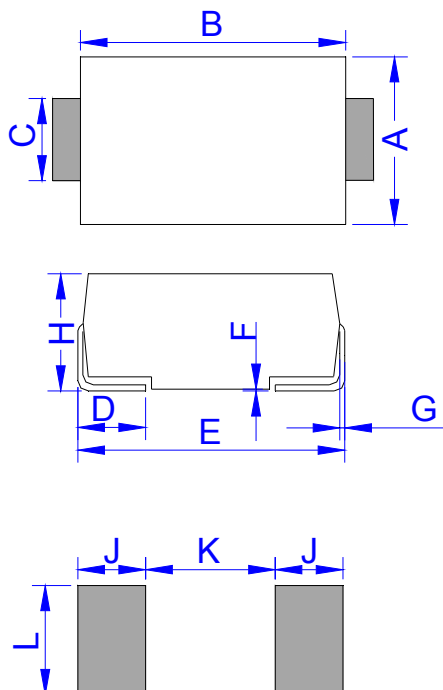
DO-214AA (SMB)
