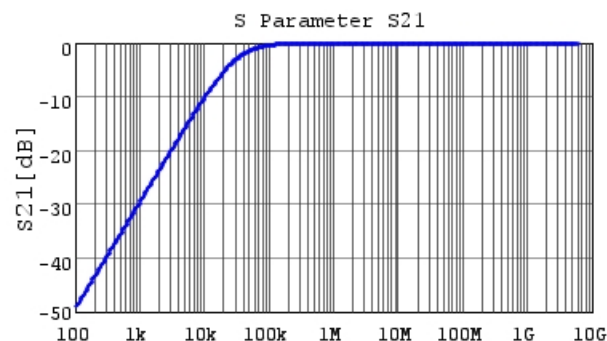
■ GRT033C80J683KE01 S21 DC0V,25degC
