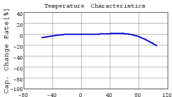
■ GRT033C80J683KE01 C-Temp. capchange, DC0.0V,
